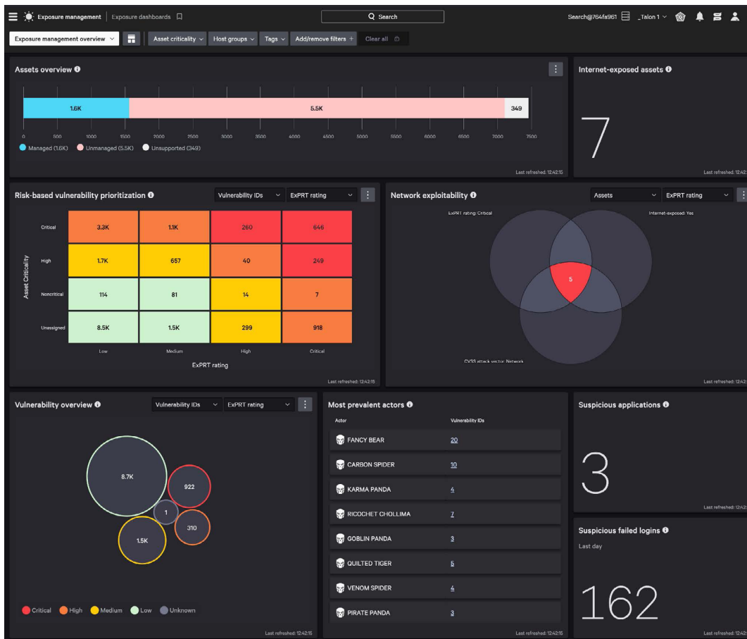
Falcon Exposure Management unified main dashboard
